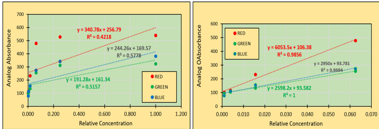
Fig. 2.a Red Color Dye 1:10 Serial Dilution with 6 Point Calibration Curve. R^2 was moderately low at 6 points; 2b. Red Color Dye 1:10 Serial Dilution with 4-Point Calibration Curve. The 4-point calculation was far higher, with R^2 near 1.
