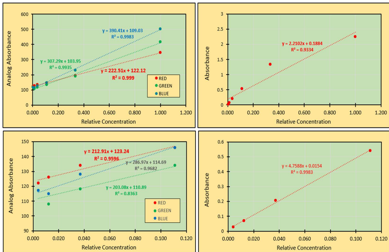
Fig. 8 presents the comparison of RGB (a;left) and commercial vis-uv spectrophotometer (b;right) with six and four-point calibration curves (1:3 turbid water serially diluted)
