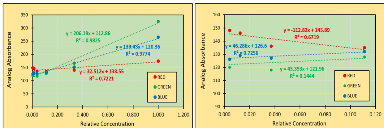
Fig. 5.a presents the analog absorbance from the 6 Point Calibration Curve of the gold colloidal solution. R^2 was higher at 6 points; b presents 4 point Calibration Curve. The 4-point calculation was less R^2 compared to the 6 points.
