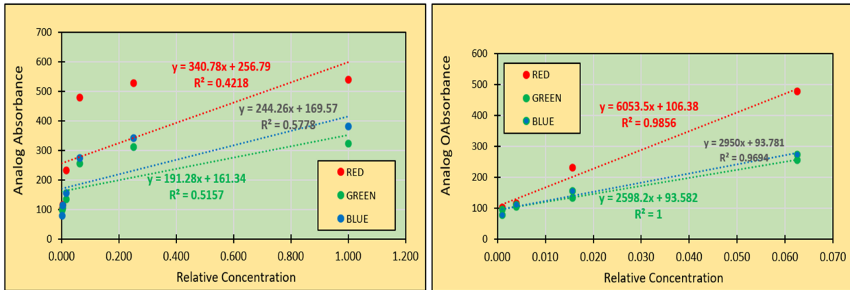
Fig. 2.a Red Color Dye 1:10 Serial Dilution with 6 Point Calibration Curve. R^2 was moderately low at 6 points; 2b. Red Color Dye 1:10 Serial Dilution with 4-Point Calibration Curve. The 4-point calculation was far higher, with R^2 near 1.
