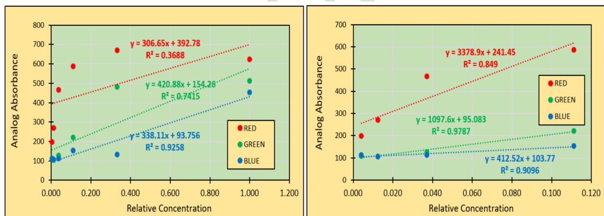
Fig. 6.a presents the analog absorbance from the 6 Point Calibration Curve of methylene blue solution. R^2 was lower at 6-points still with R squared 0.926 high; b presents 4-point Calibration Curve. The 4-point calculation had a higher R^2 compared to the 6-point calculation.
