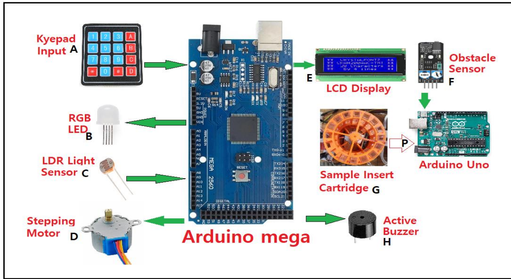
Diagram 1 presents the arrangement of our Arduino microcontroller with the sensors and actuators used in this project.
