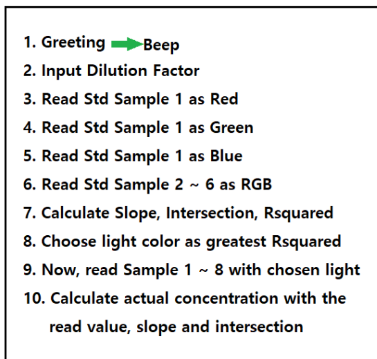
Diagram 2 illustrates the flow diagram of our software and algorithm.
