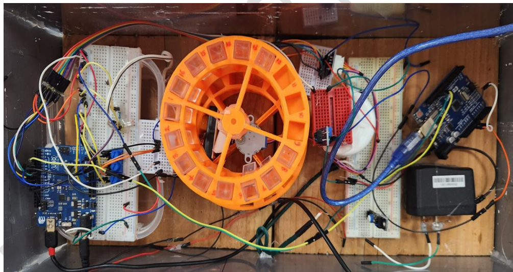
Fig.1 presents the pictorial representation of our completed project assembly as described above.
