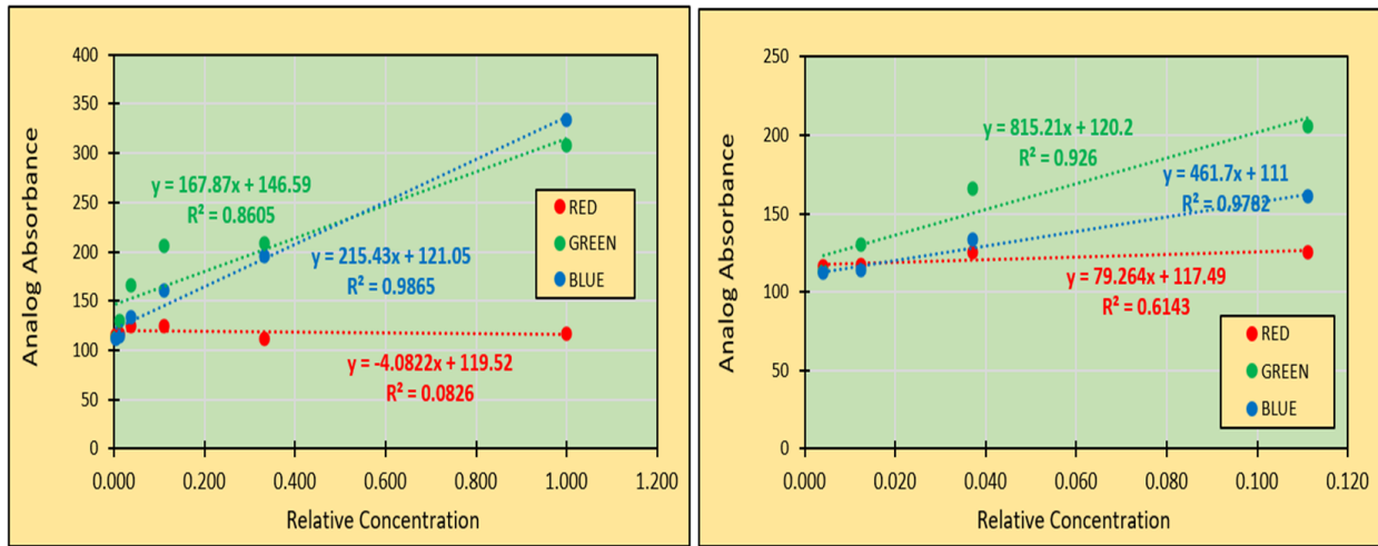
Fig. 7.a presents the analog absorbance from the 6 Point Calibration Curve of methylene blue solution. R2 was lower at 6-points still with R squared 0.987 high; b presents a 4-point Calibration Curve. The 4-point calculation had a lower R2 compared to the 6-point calculation.
