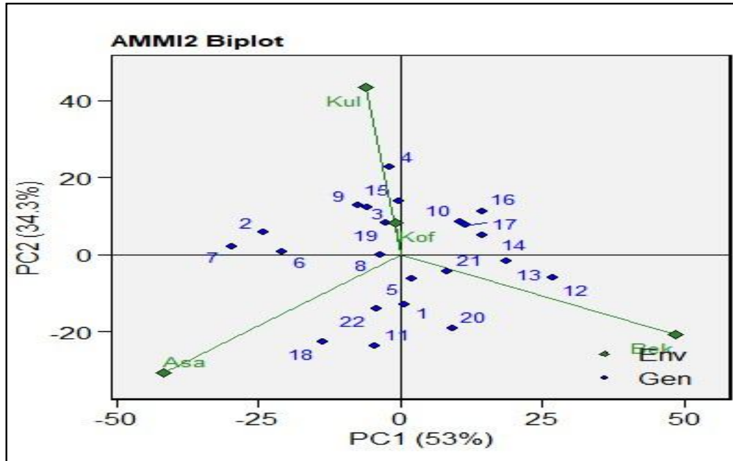
Figure 1: AMMI2
