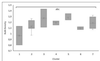
(m) BD
