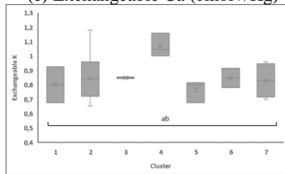
(h) Exchangeable K (cmol+/Kg)
