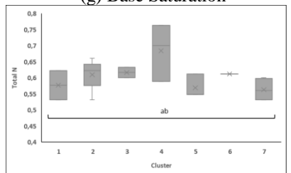
(j) Total N
