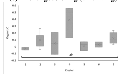
(f) Organic C
