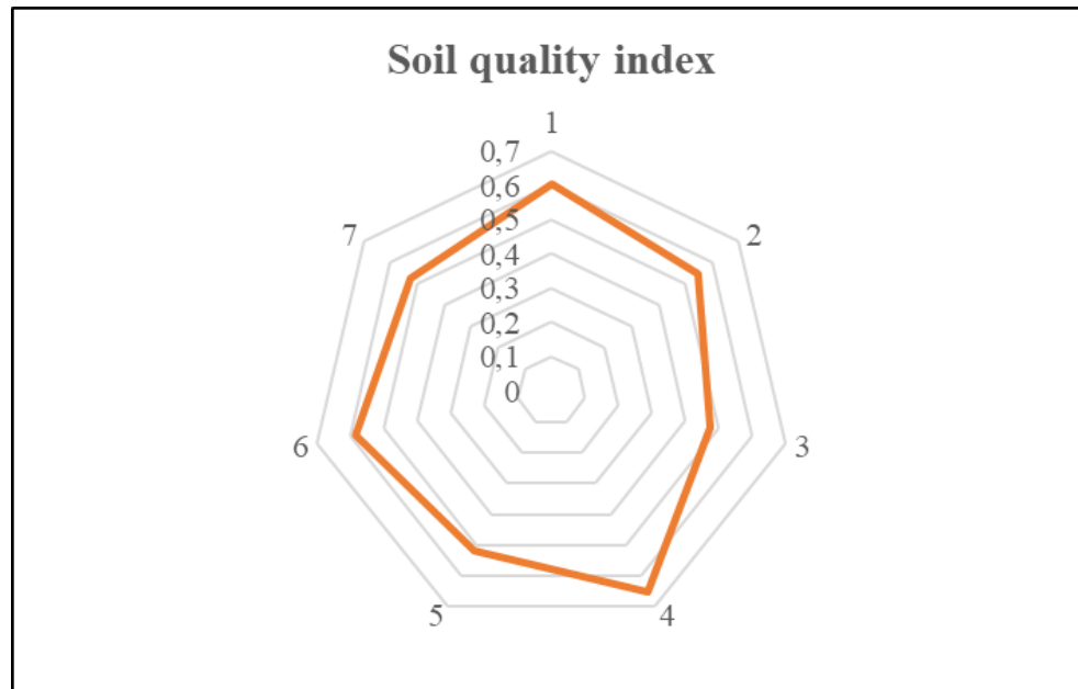
Figure 5. Diagram hexagon of soil quality indeks
