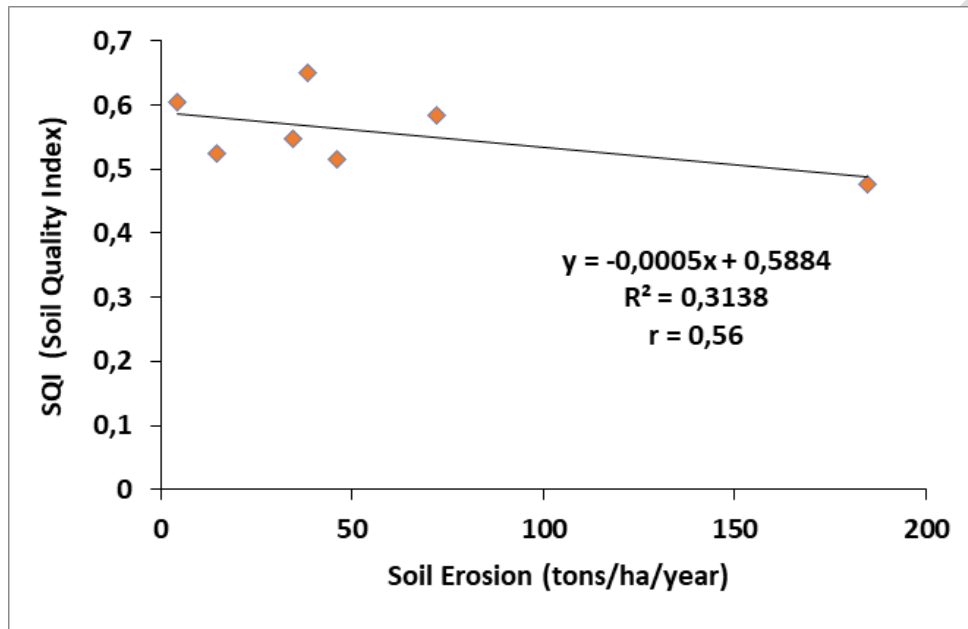
Figure 6. Correlation between soil erosion and soil quality index
