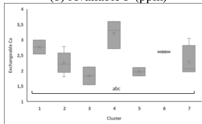
(e) Exchangeable Ca (cmol+/Kg)
