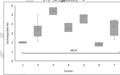
(i) Exchangeable Na (cmol+/Kg)
