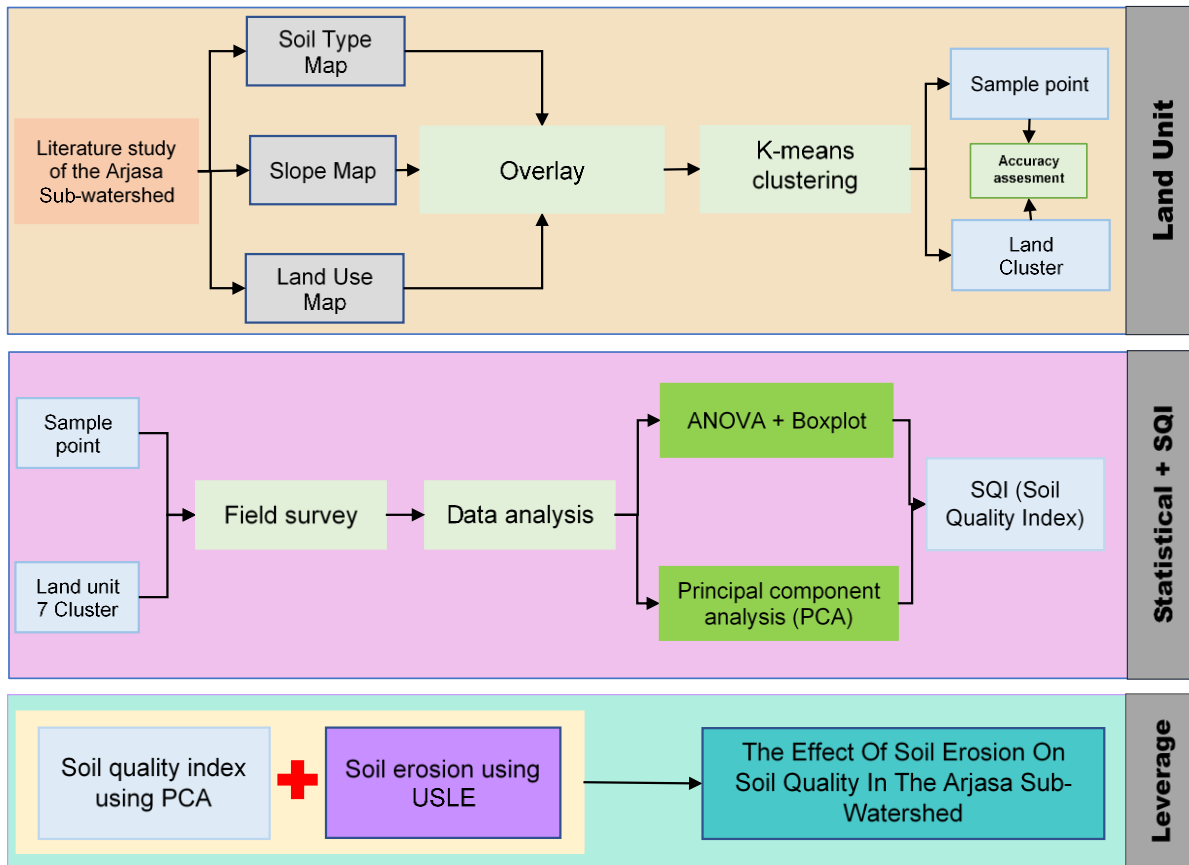
Figure 3 Research framework
