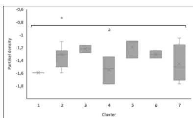
(p) PD
