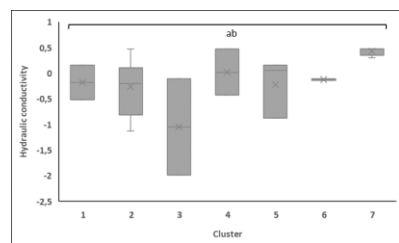
(n) Hydraulic conductivity
