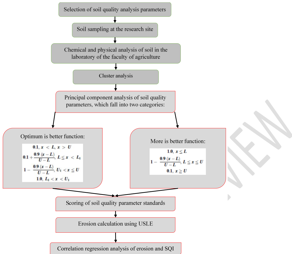
Figure 2 Research framework
